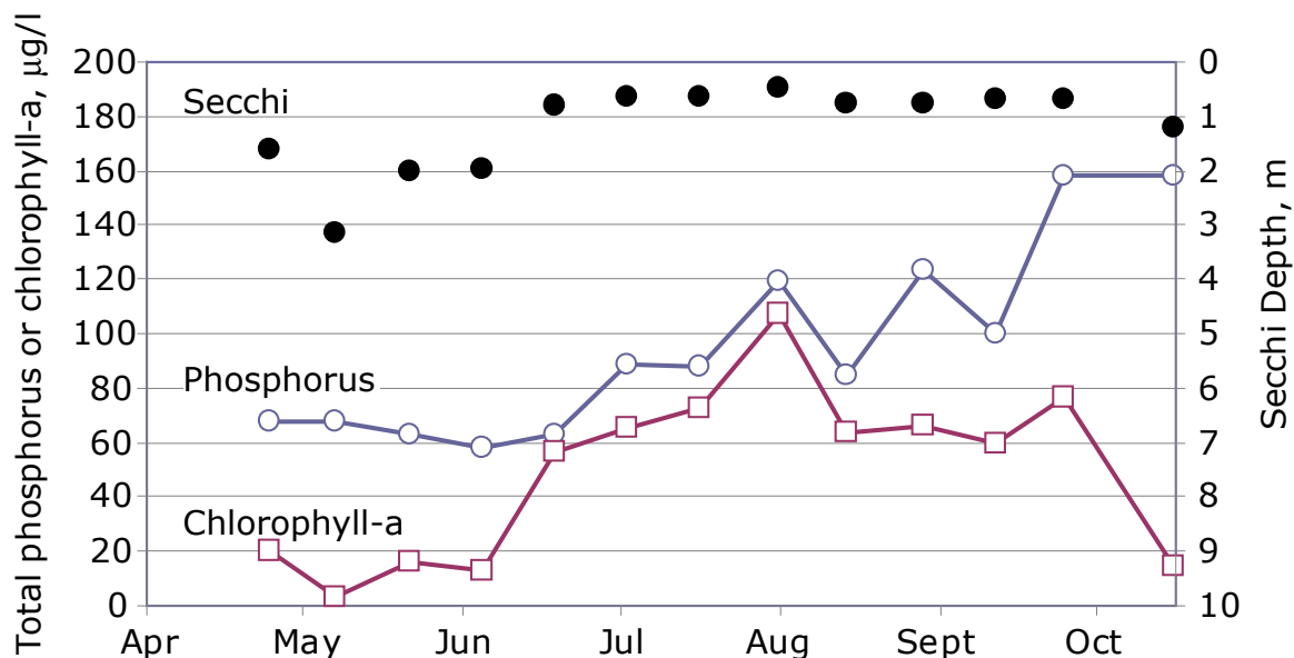
Figure 1.7. Bi-weekly monitoring data from 2007 for Lake Sarah showing typical annual variations of secchi depth, total phosphorus, and chlorophyll-a.
